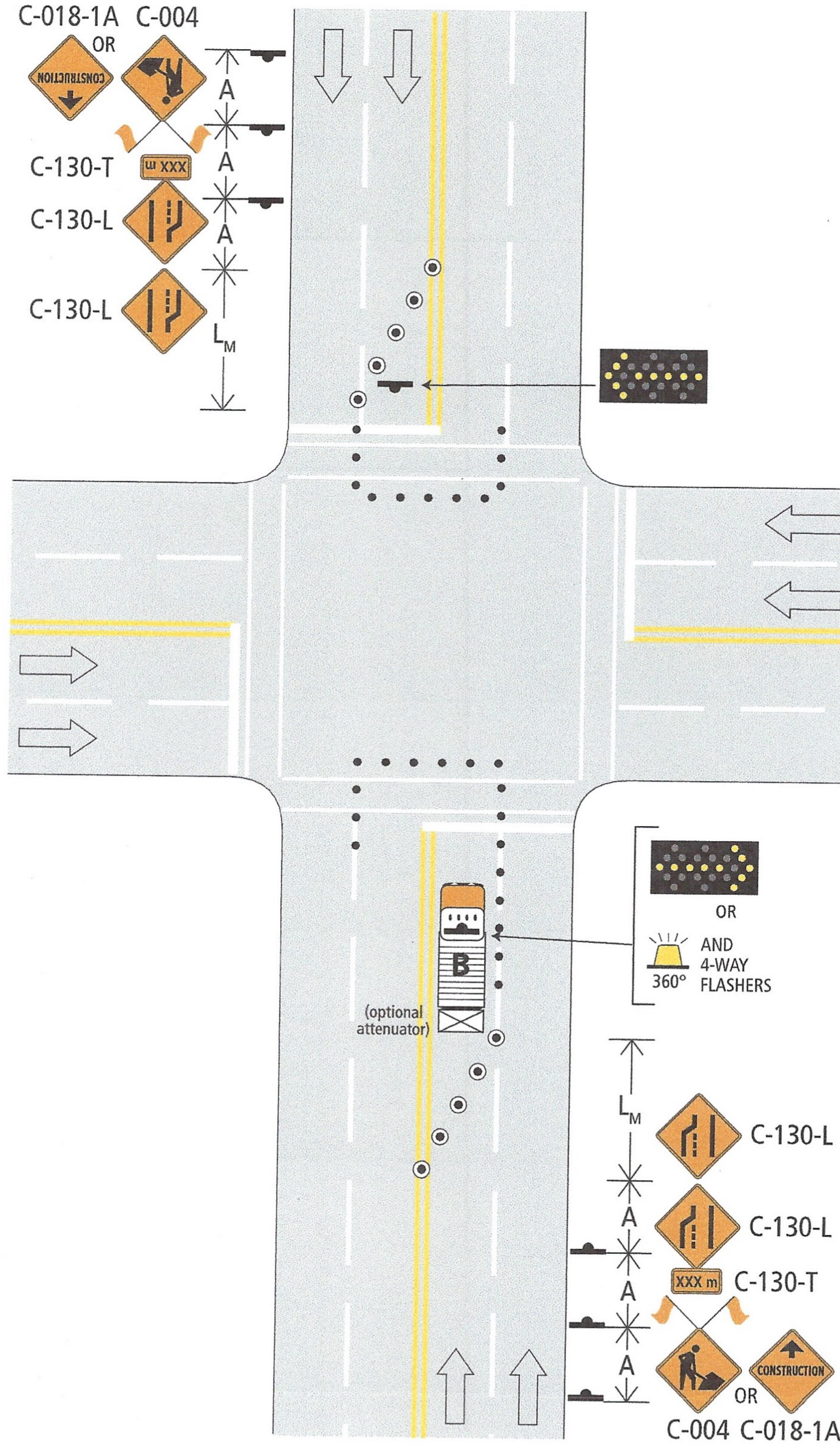
Figure 14.10: Stop Line and Crosswalk Marking – Left Lanes – Multilane Roadway – Short and Long Duration
